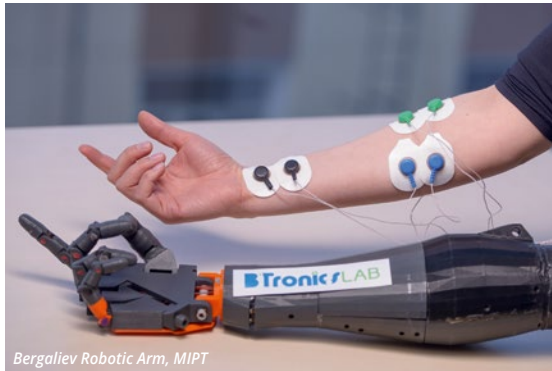
Bergaliev Robotic Arm, MIPT
